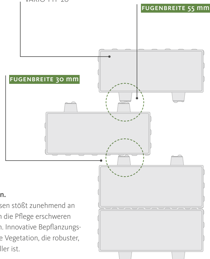
VEGETATIONSFUGENSTEIN VARIO TYP 20
